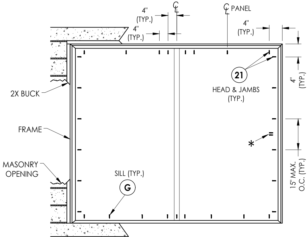
FRAME ANCHORING 2X BUCK
