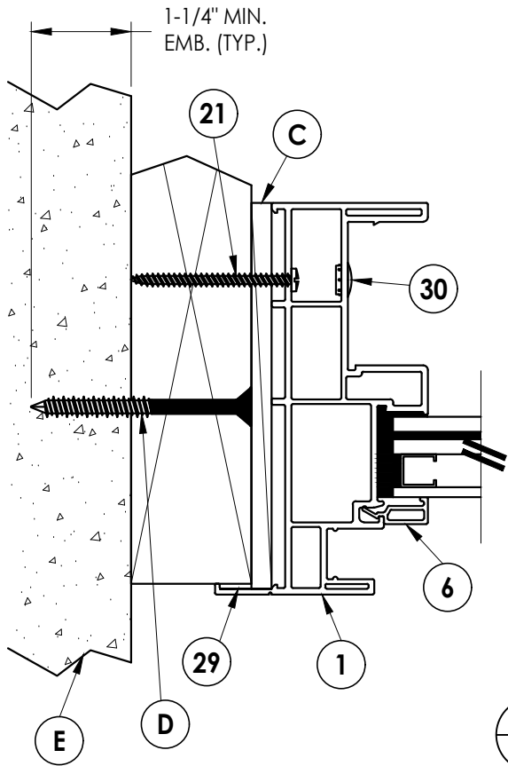
HORIZONTAL CROSS SECTION
