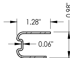
10 M JAMB STILE (PD25) Reinforcement Roll formed steel
