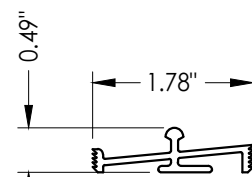
8 SILL TRACK Extruded aluminum
