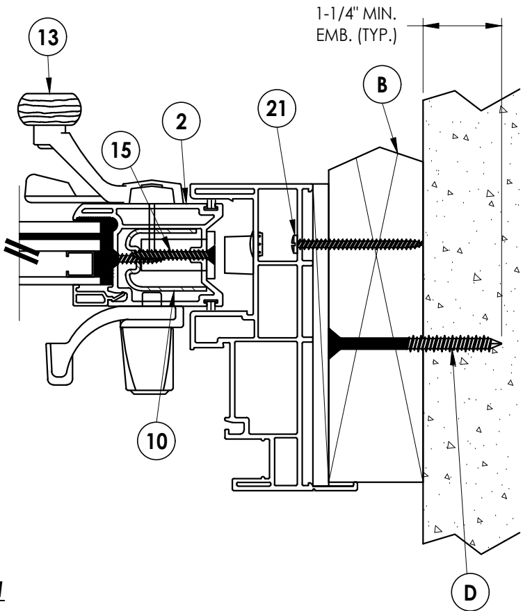
HORIZONTAL CROSS SECTION
