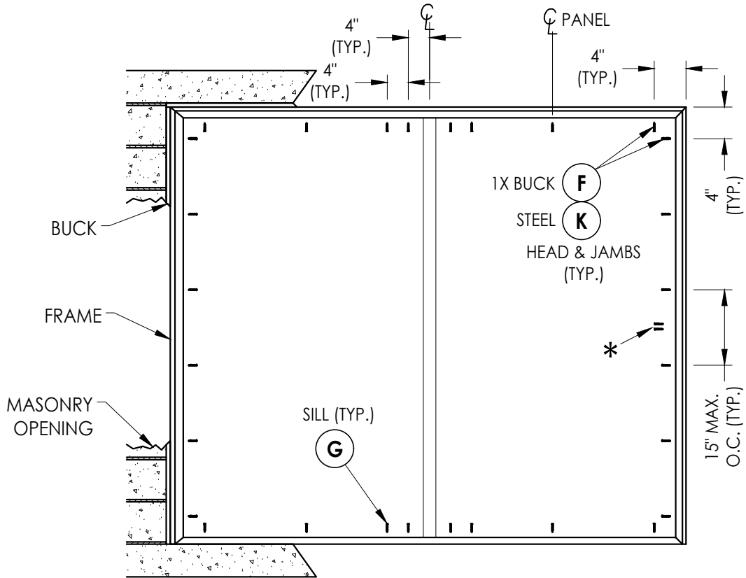
FRAME ANCHORING 1X BUCK
