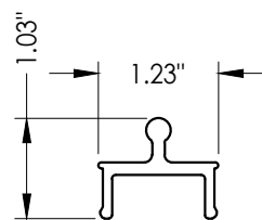
28 SCREEN TRACK Extruded vinyl
