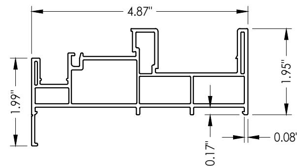
1 HEAD / SILL / JAMB Extruded vinyl
