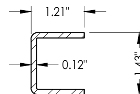
12 FIXED INTERLOCK (PD34) Roll formed steel
