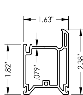
2 STILE / RAIL Extruded vinyl
